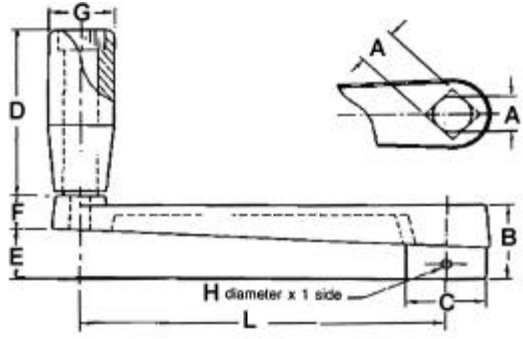
WITH PLASTIC REVOLVING HANDLE
