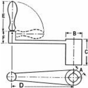
Broached, Plain or Custom Broached to Customer specs.
