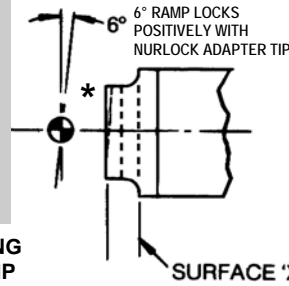
TYPE HNL-1
