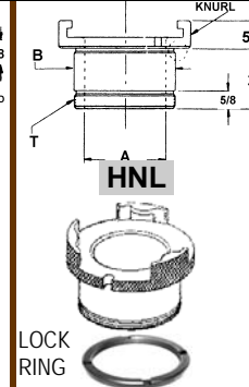
KNURLED O.D. +.025 +.010
