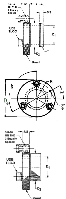
STANDARD LOCK LL
