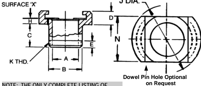
TYPE HNL
