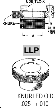
LOCK RING
